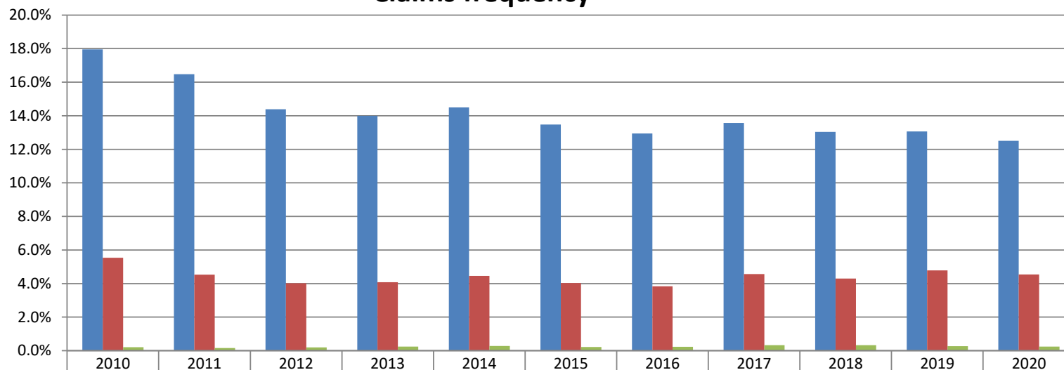
Claims frequency
