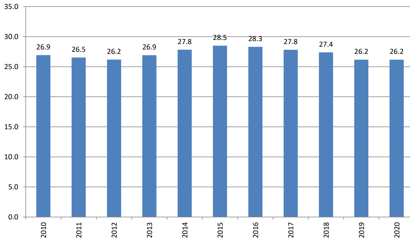
Average age
